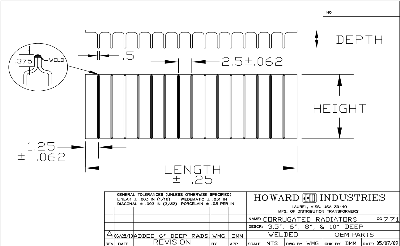
Figure 1: Outline drawing of 3.5", 6", 8" and 10" depth corrugated radiators
