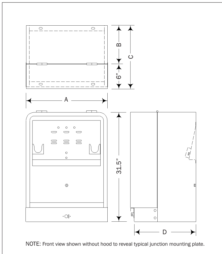
FIGURE 1: Dimensions for standard single-phase style junction enclosures (refer to Table 1)
