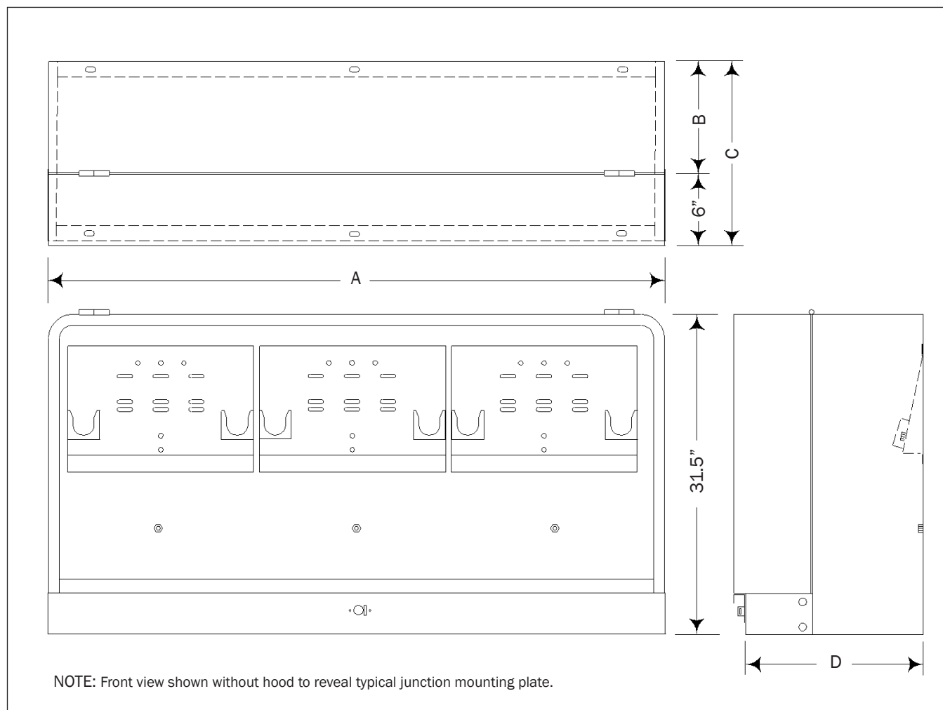
FIGURE 2: Dimensions for standard three-phase style junction enclosures (refer to Table 2)
