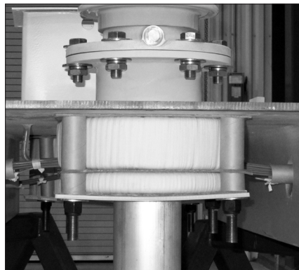
Figure 16: CTs mounted under cover
