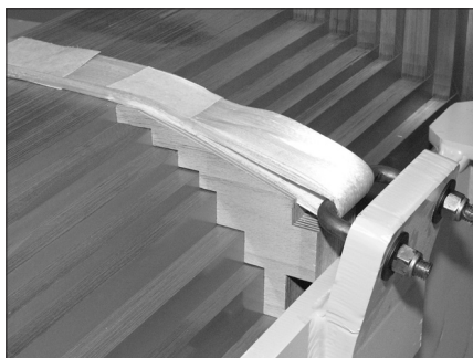
Figure 7: Core support blocks
