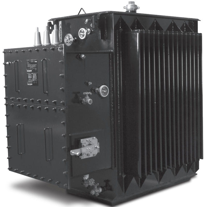
Figure 1: Network Transformer
