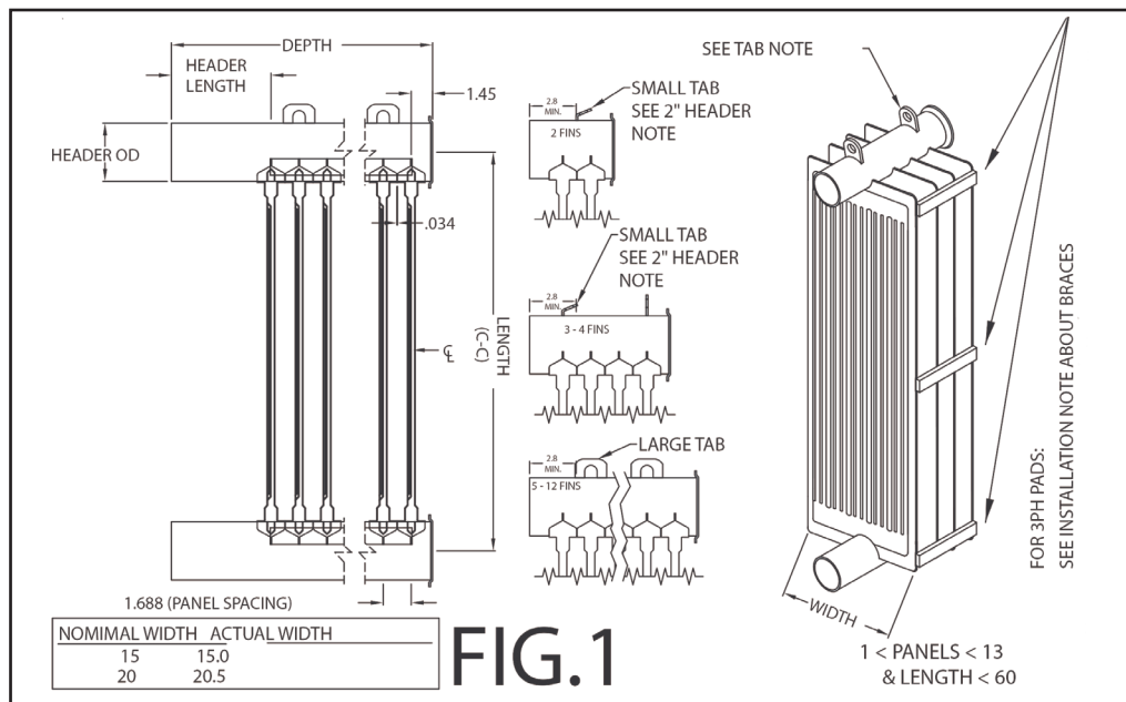
FIGURE 1: Panel Radiator, Length \leq 59" and Number of Panels \leq 12
