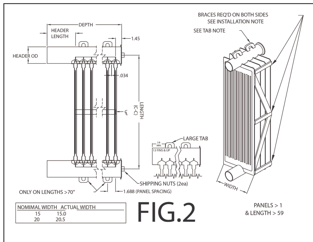
FIGURE 2: Panel Radiator, Length \geq 60" and Number of Panels \geq 13
